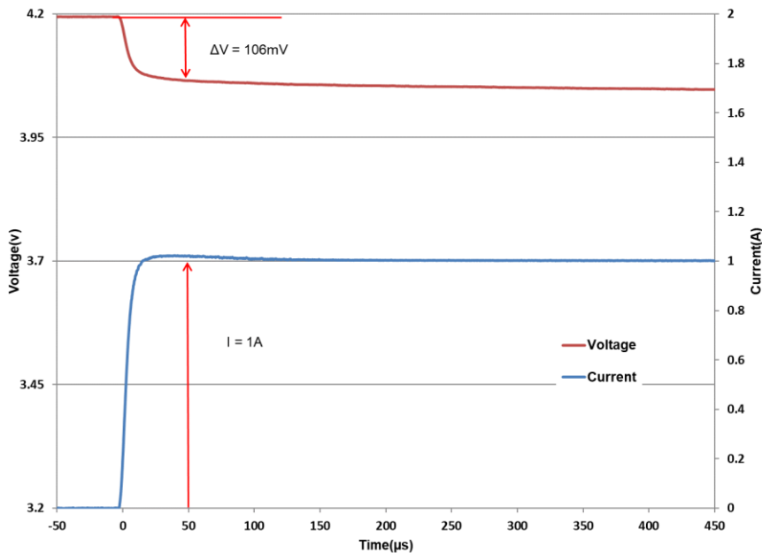
Fig 3: Measurement of ESR for a DMT334R2S474M3DTA0
