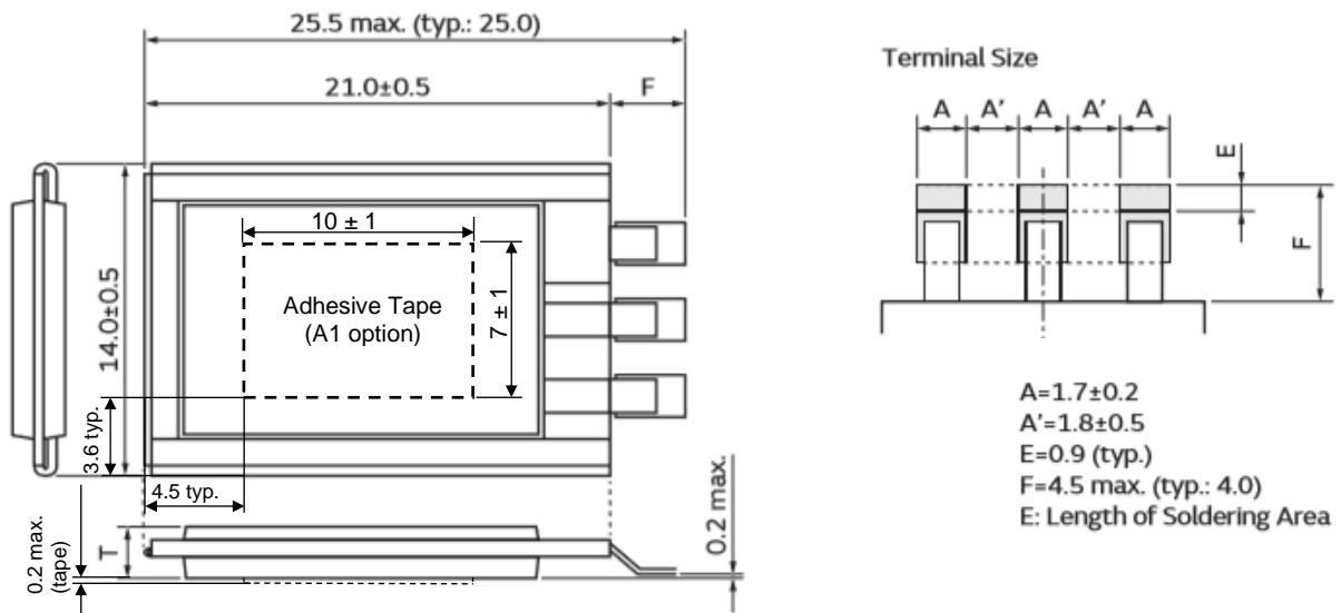
Mechanical drawing for DMT334R2S474M3DTA0
