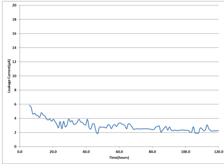
Fig 10: Leakage Current
